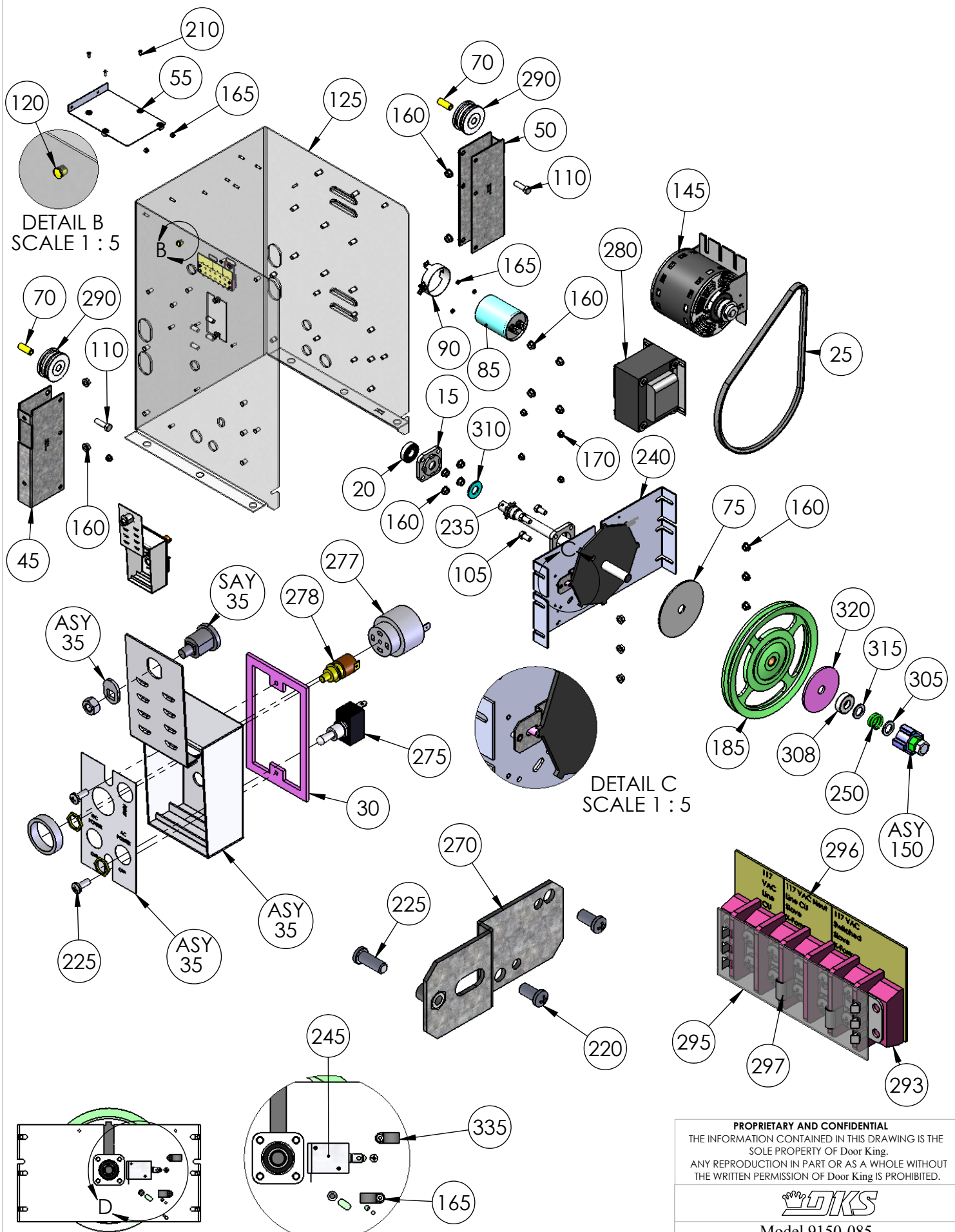
DETAIL D SCALE 1 : 6
