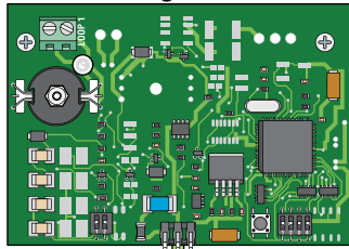
Plug-In Loop Detector 9410 Single Channel
